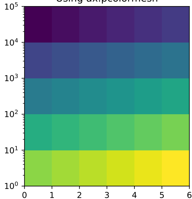
Using ax.pcolormesh
